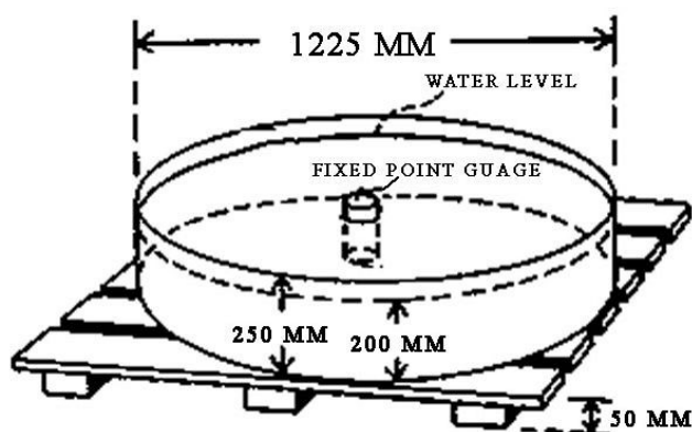
Figure 1 – Class A Evaporation Pan Installed on a Wooden Platform
