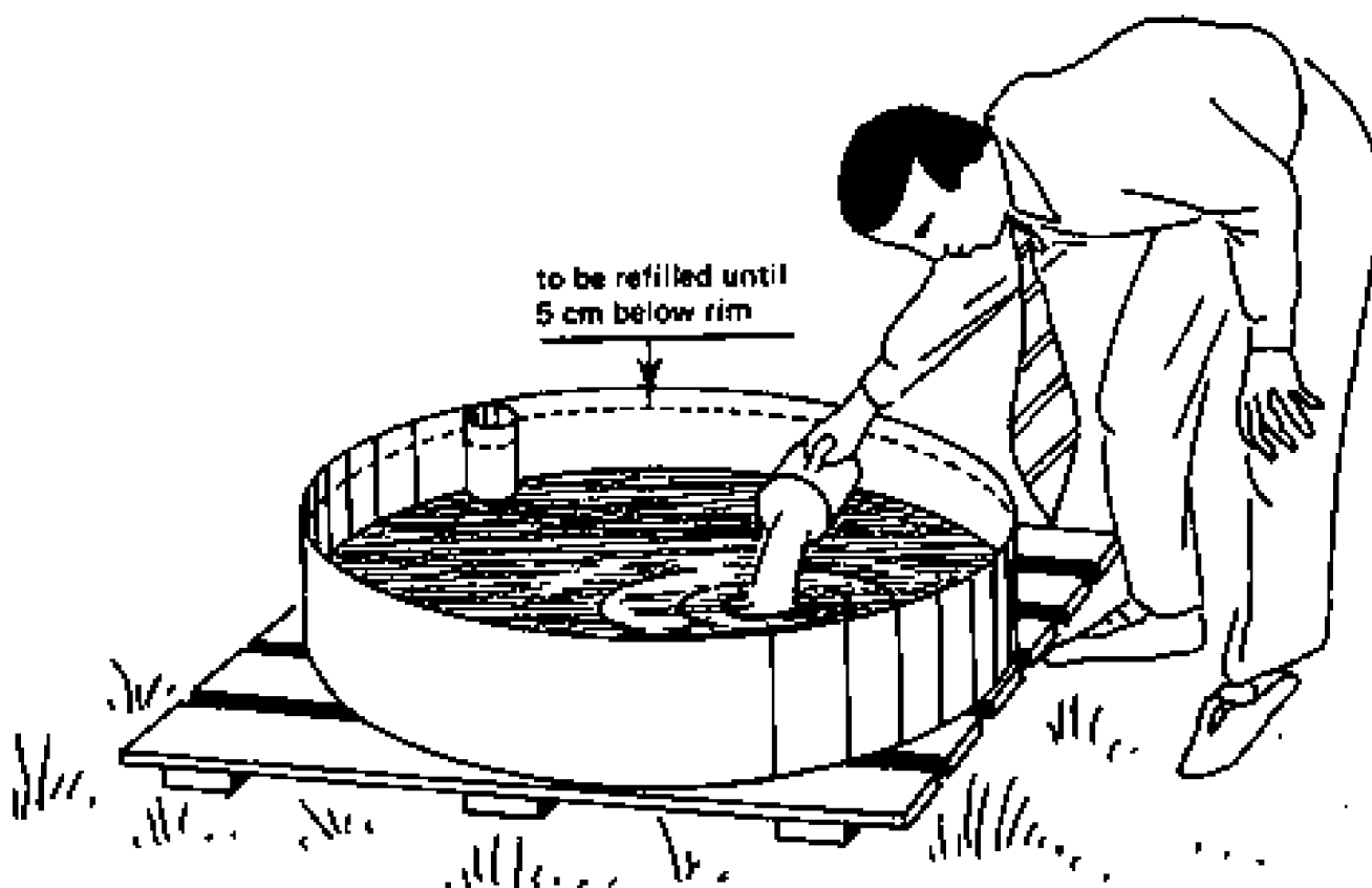
Figure 2 – Refilling water to the fixed point gauge (datum).
