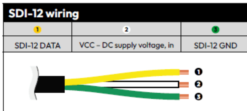
Figure 6 – Cable Pinout
